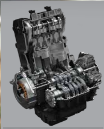
776cm³, 4-stroke, 2-cylinder, Liquid-cooled, DOHC, Parallel Twin Engine
